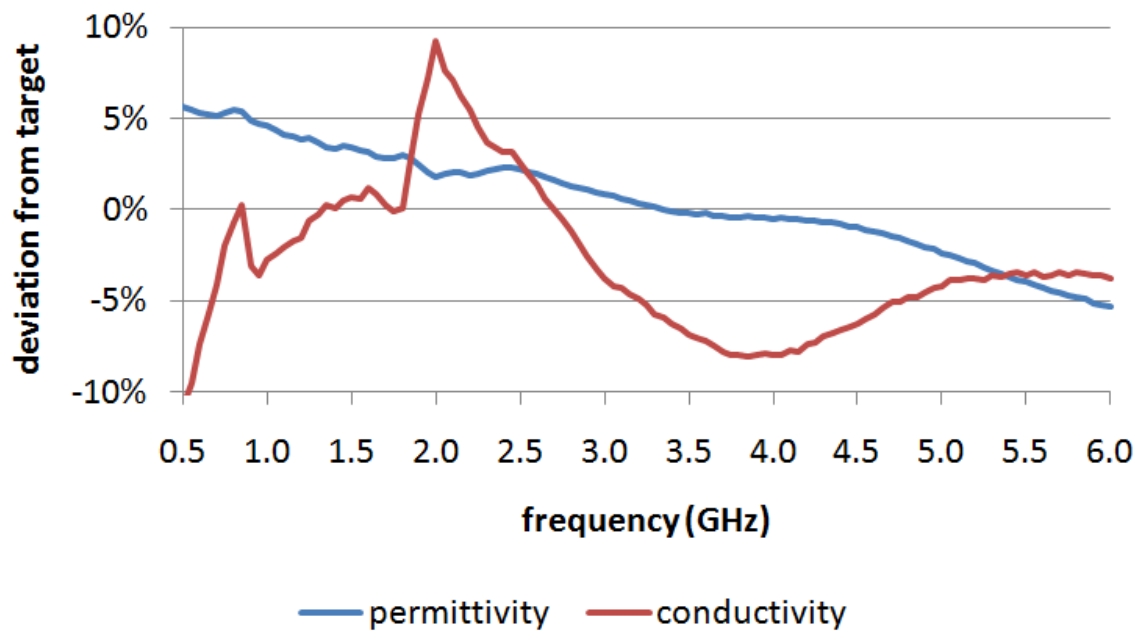
Figure 1: Typical permittivity and conductivity values of the iSAR dielectric medium for head tissue versus frequency. The values are expressed as a percent deviation from the target dielectric parameters specified in IEEE 1528 and IEC 62209-2. The values are within an acceptable 10% tolerance of the target values, as specified in IEC 62209-2.
